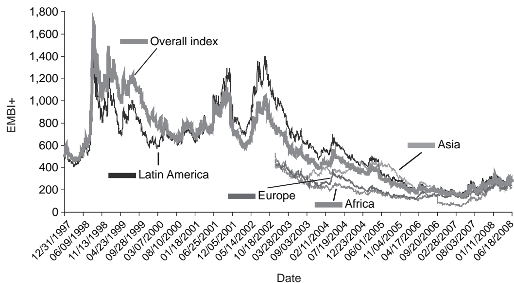
Figure 6: EMBI+ Spreads
